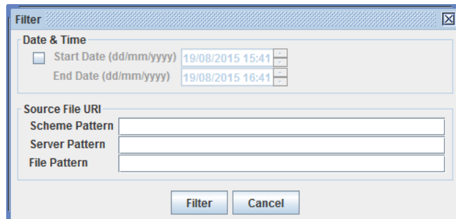
Figure 9.2: Filter
