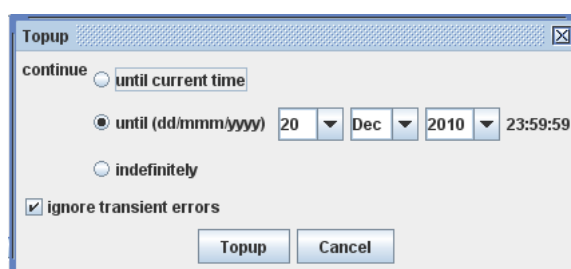
Figure 9.4: Topup
