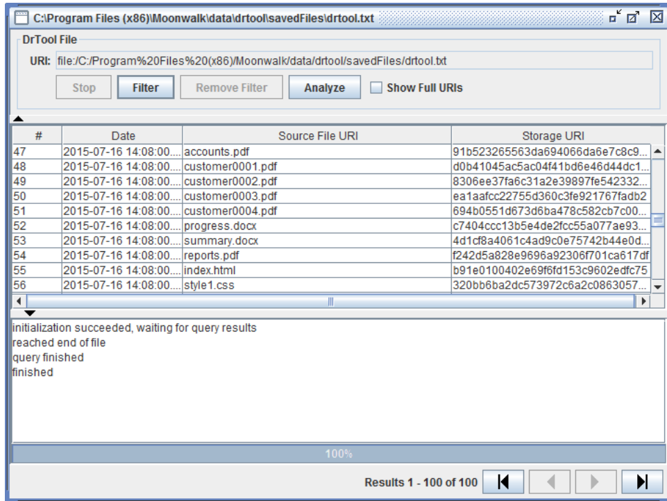
Figure 9.1: Results Window
