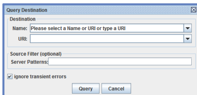
Figure 9.3: New Query
